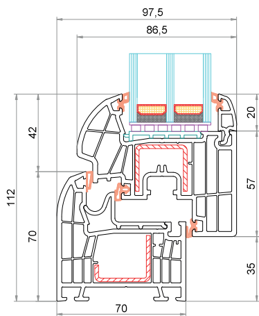
Telaio CK-L001 Anta CK-Z003
