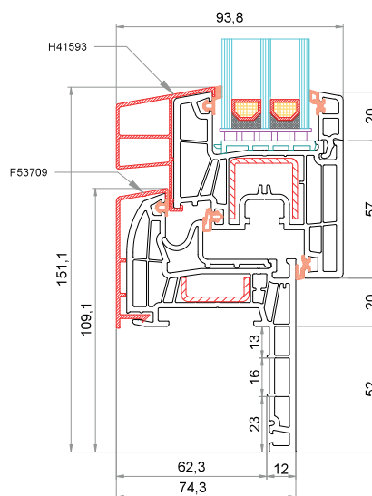
Telaio Reno 52 mm CK-L029 + AluClip F53709 Anta CK-Z051 + AluClip H41593
