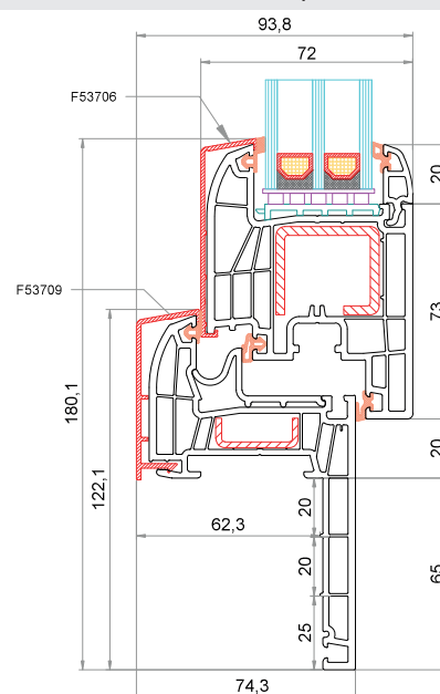
Telaio Reno 30 mm CK-L031 + AluClip F53709 Anta CK-Z041 + AluClip F53706
