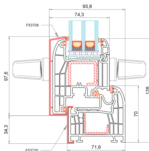
Telaio CK-L001 + AluClip F53720 Anta CK-Z040 (maniglia passante) + AluClip F53708
