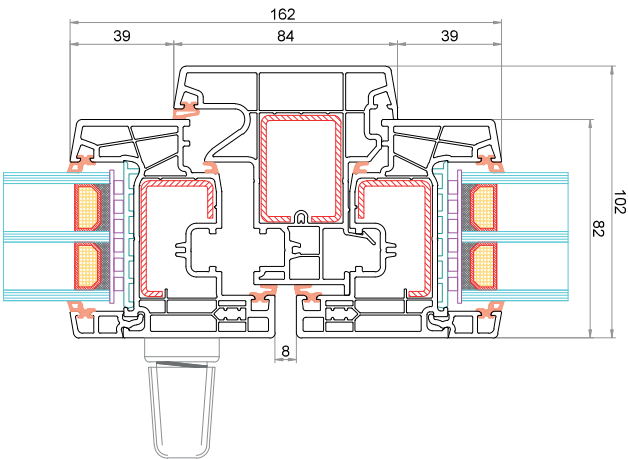
Anta CK-Z801 Battente mobile 84 mm CK-T884 Anta CK-Z801
