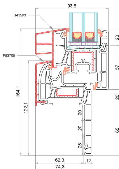
Telaio Reno 65 mm CK-L065 + AluClip F53709 Anta CK-Z051 + AluClip H41593
