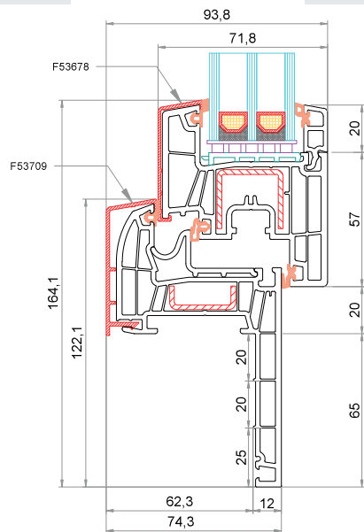
Telaio Reno 65 mm CK-L065 + AluClip F53709 Anta CK-Z051 + AluClip F53678
