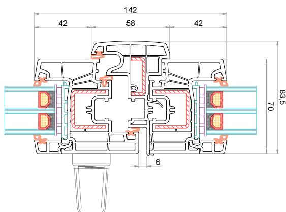
Anta CK-Z051 Battente mobile 58 mm CK-T046 Anta CK-Z051
