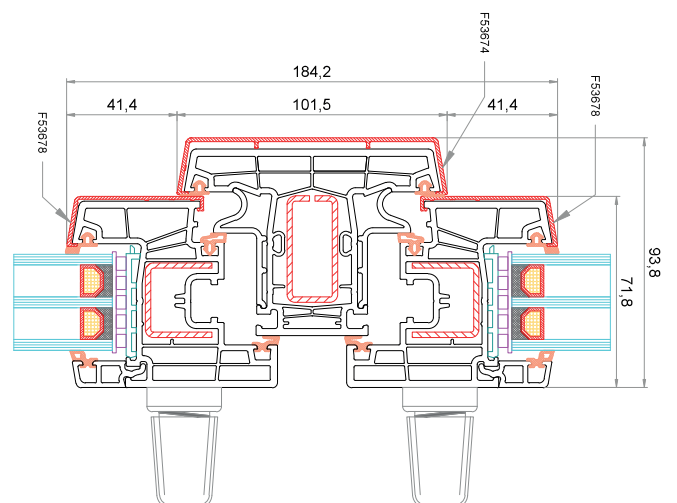
Anta CK-Z051 + AluClip F53678 Montante fisso da 96 mm CK-T050 + AluClip F53674 Anta CK-Z051 + AluClip F53678
