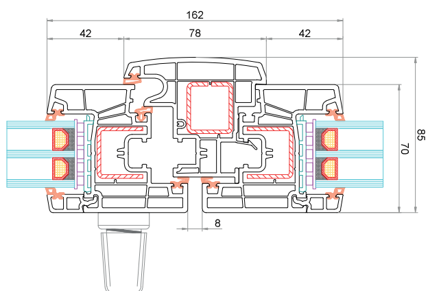
Anta CK-Z051 Battente mobile 78 mm CK-T045 Anta CK-Z051
