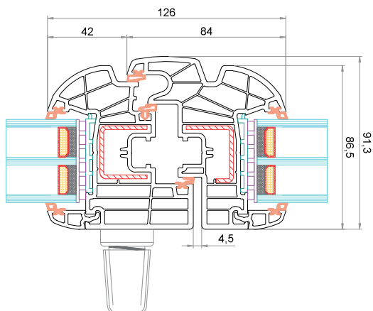
Anta CK-Z003 Anta - montante mobile 84 mm CK-Z030
