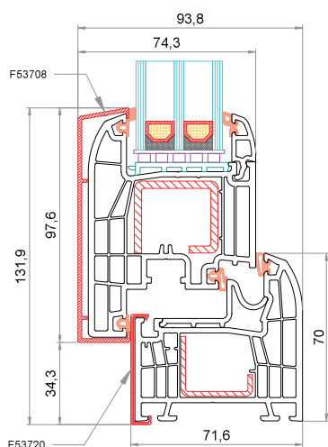
Telaio CK-L001 + AluClip F53720 Anta CK-Z040 + AluClip F53708
