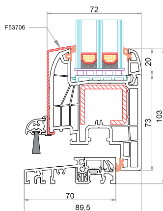
Anta CK-Z041 + AluClip F53706 Soglia bassa 6-37852-60-0-1
