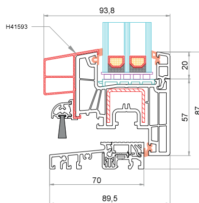
Anta CK-Z051 + AluClip H41593 Soglia bassa 6-37852-60-0-1
