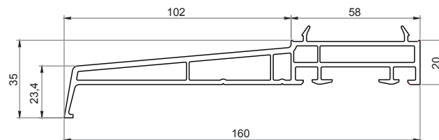
Davanzale 102 mm FB102
