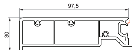
Tapee 97.5 mm 27TA9730
