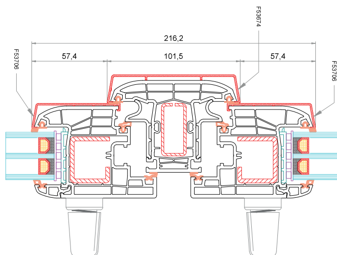
Anta CK-Z041 + AluClip F53706 Montante fisso da 96 mm CK-T004 + AluClip F53674 Anta CK-Z041 + AluClip F53706
