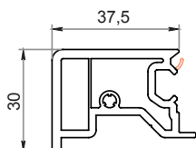
Tapee 37.5 mm 27TA3730
