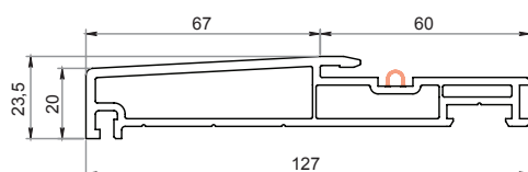
Davanzale 67 mm 6136
