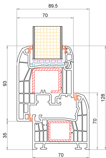
Telaio CK-L001 Anta CK-Z040
