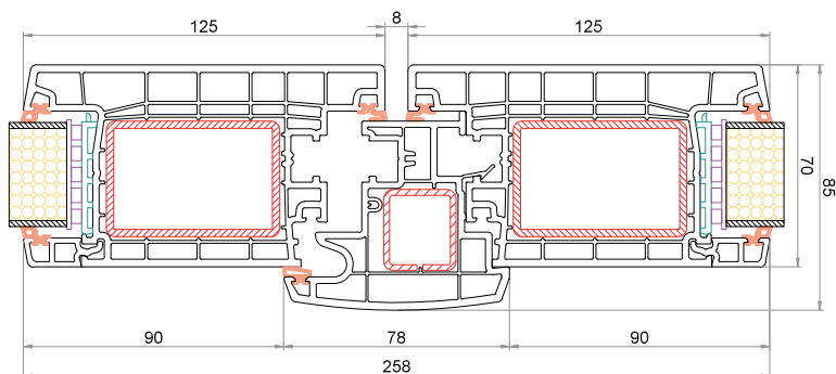
Anta CK-Z056 Battente mobile 78 mm CK-T045 Anta CK-Z056
