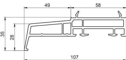
Davanzale 49 mm FB49
