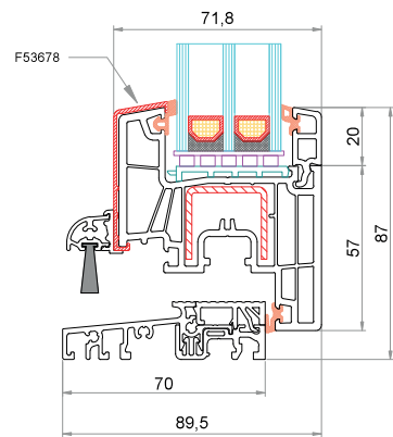
Anta CK-Z051 + AluClip F53678 Soglia bassa 6-37852-60-0-1
