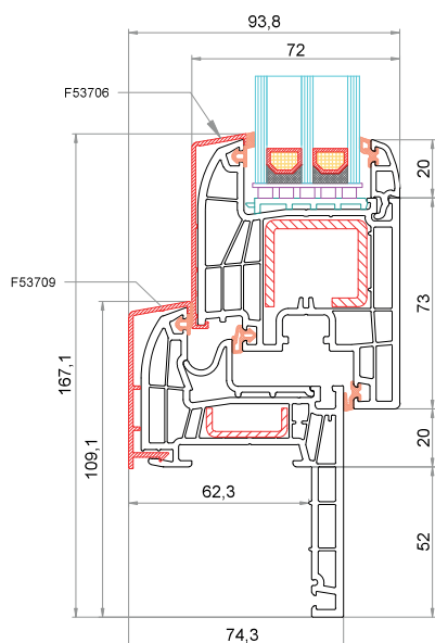
Telaio Reno 52 mm CK-L029 + AluClip F53709 Anta CK-Z041 + AluClip F53706
