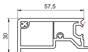
Tapee 57.5 mm 27TA5730
