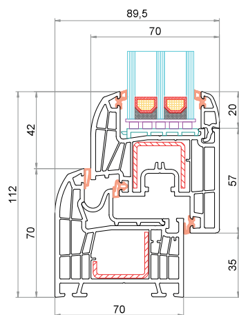
Telaio CK-L001 Anta CK-Z044
