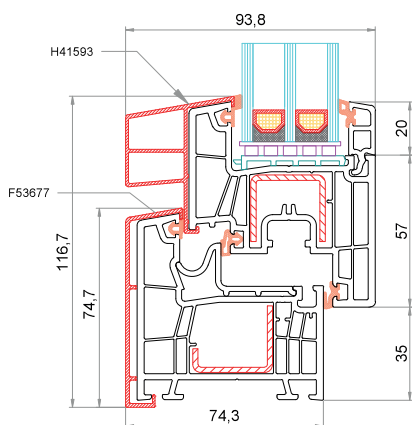
Telaio CK-L052 + AluClip F53677 Anta CK-Z051 + AluClip H41593
