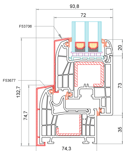
Telaio CK-L001 + AluClip F53677 Anta CK-Z041 + AluClip F53706
