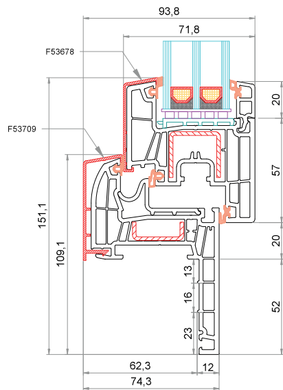
Telaio Reno 52 mm CK-L029 + AluClip F53709 Anta CK-Z051 + AluClip F53678
