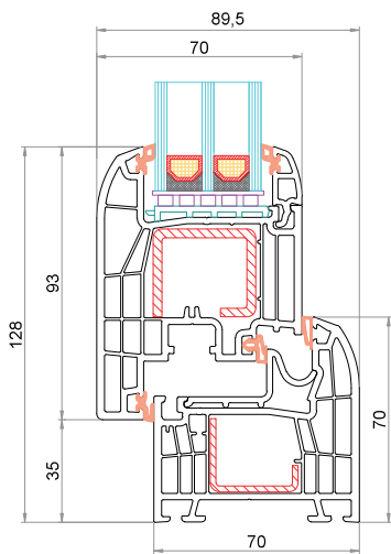
Telaio CK-L001 Anta CK-Z040
