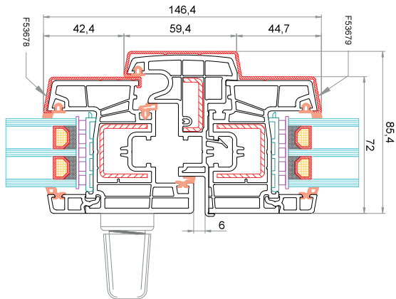
Anta CK-Z051+ AluClip F53678 Battente mobile 58 mm CK-T046 Anta CK-Z051 + AluClip F53679
