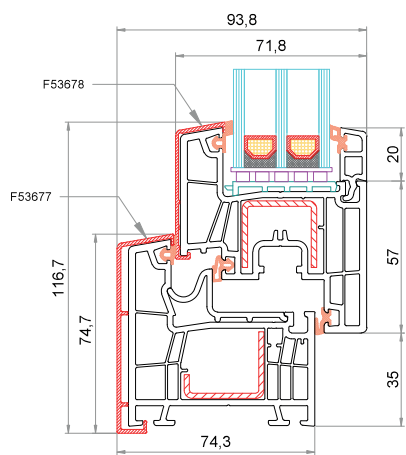
Telaio CK-L052 + AluClip F53677 Anta CK-Z051 + AluClip F53678
