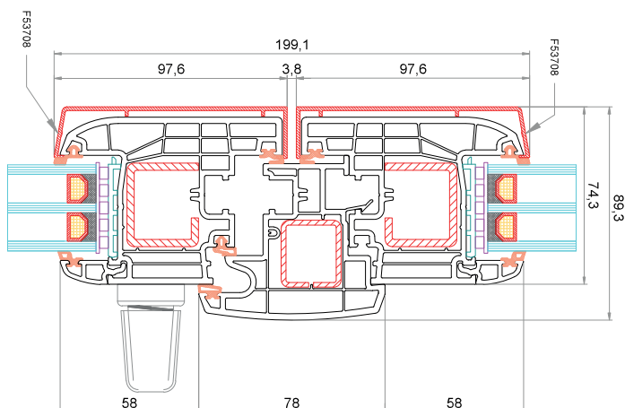
Anta CK-Z040 + AluClip F53708 Battente mobile 78 mm CK-T045 Anta CK-Z040 + AluClip F53708
