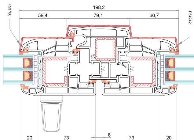
Anta CK-Z041 + AluClip F53706 Battente mobile 78 mm CK-T045 Anta CK-Z041 + AluClip F54242
