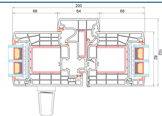
Anta CK-Z841 Battente mobile 64 mm CK-T864 Anta CK-Z841
