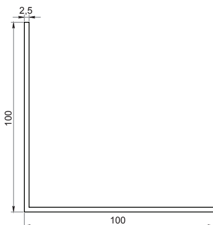
Barra angolare 100x100 mm 25CR100100
