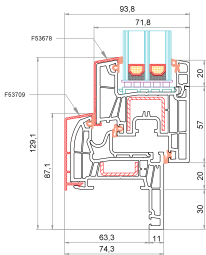
Telaio Reno 30 mm CK-L031 + AluClip F53709 Anta CK-Z051 + AluClip F53678
