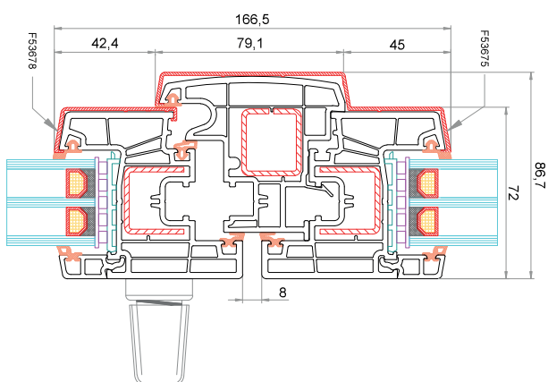
Anta CK-Z051 + AluClip F53678 Battente mobile 78 mm CK-T045 Anta CK-Z051 + AluClip F53675
