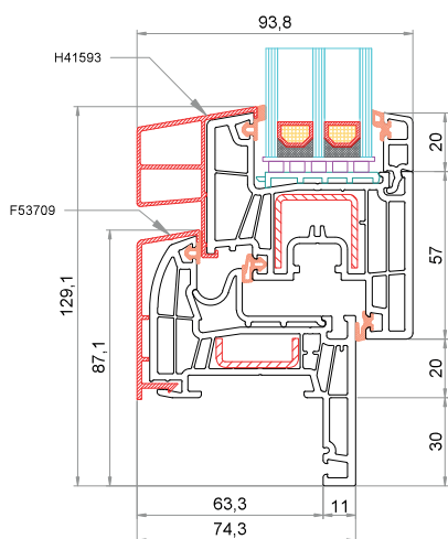
Telaio Reno 30 mm CK-L031 + AluClip F53709 Anta CK-Z051 + AluClip H41593
