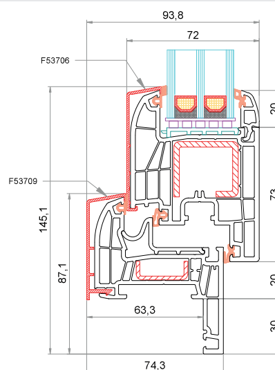
Telaio Reno 30 mm CK-L031 + AluClip F53709 Anta CK-Z041 + AluClip F53706
