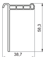
Profilo Fench CK-E066
