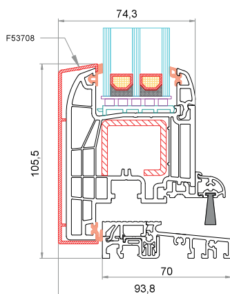
Anta CK-Z040 + AluClip F53708 Soglia bassa 6-37852-60-0-1
