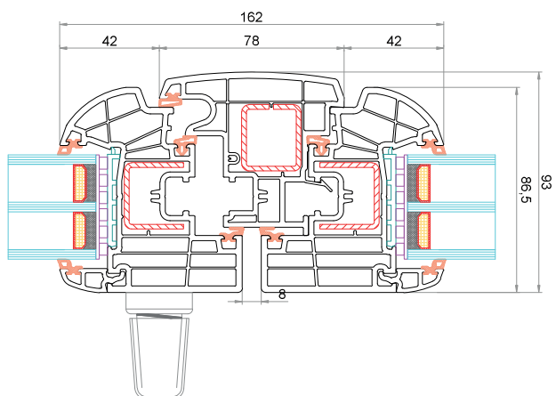
Anta CK-Z003 Battente mobile 78 mm CK-T045 Anta CK-Z003
